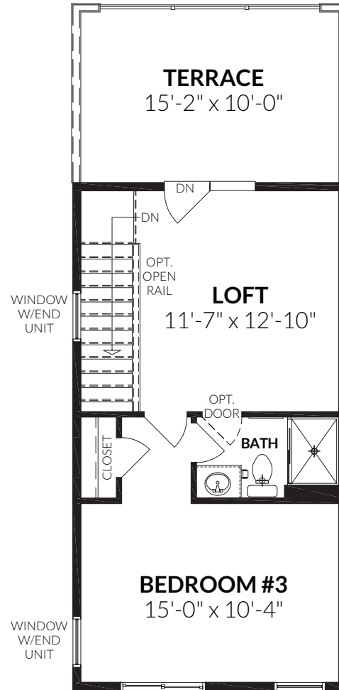
LOFT FLOOR (REAR TERRACE)
