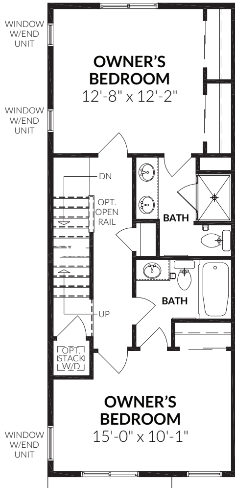
SECOND FLOOR (ELEVATION 1)
