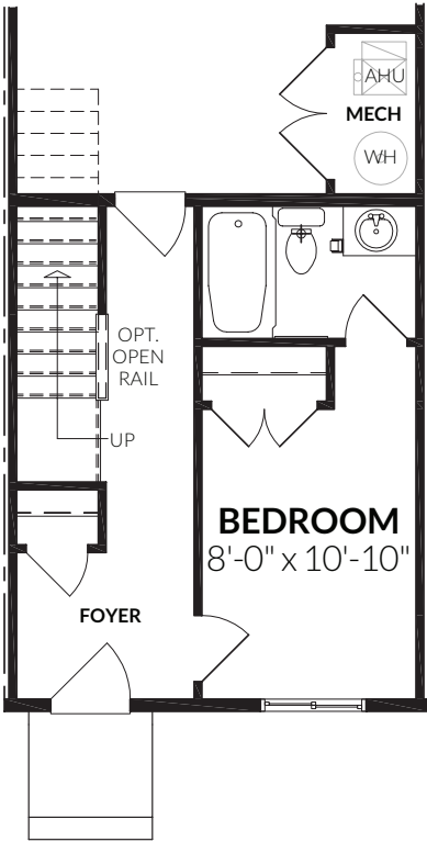
GROUND LEVEL WITH BEDROOM AND FULL BATH (ELEVATION 2 & 3)
