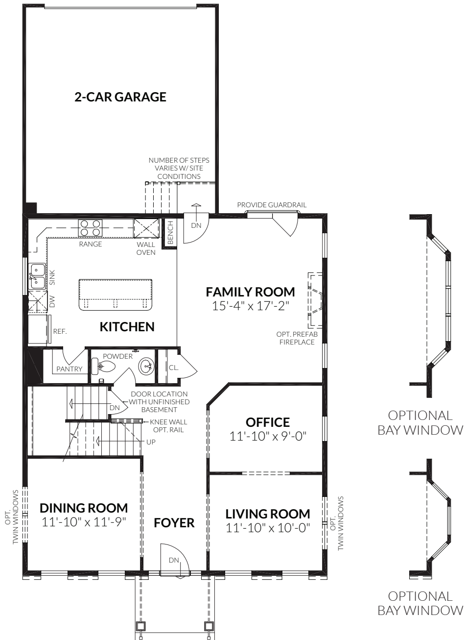
ALTERNATE FIRST FLOOR
