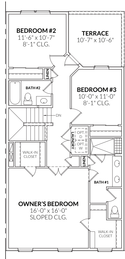
FOURTH FLOOR PLAN WITH OPTIONAL TERRACE
