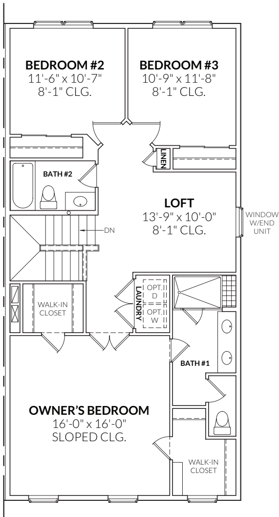
FOURTH FLOOR PLAN ELEVATIONS #1, #2 & #3
