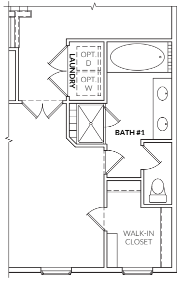
PARTIAL FLOOR PLAN WITH OPT. DELUXE BATH
