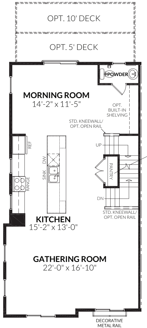
FIRST FLOOR (END UNIT)
