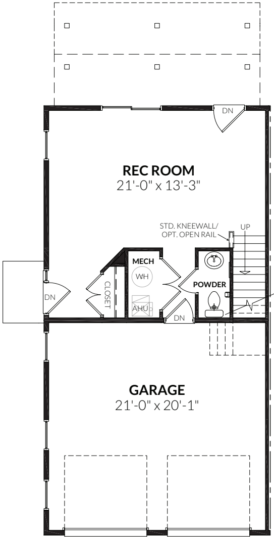
GROUND LEVEL (END UNIT)
