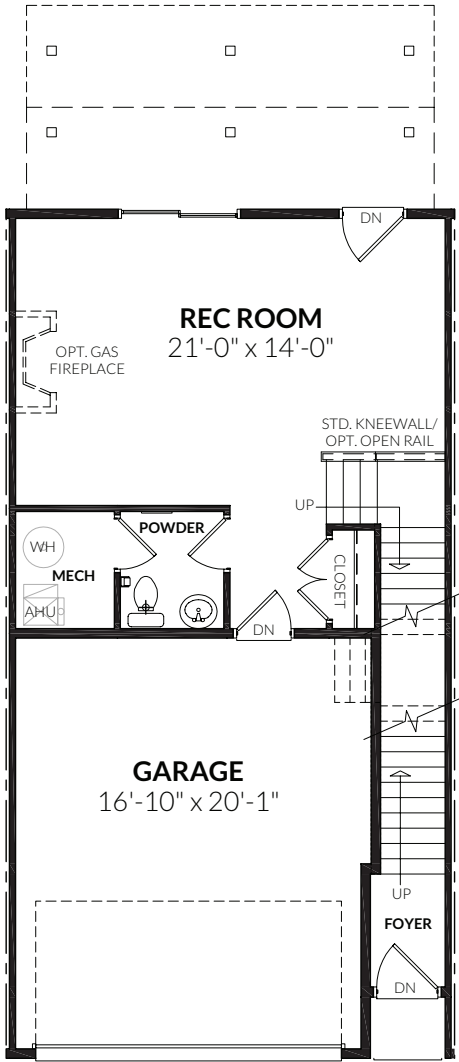
GROUND LEVEL (INTERIOR UNIT)
