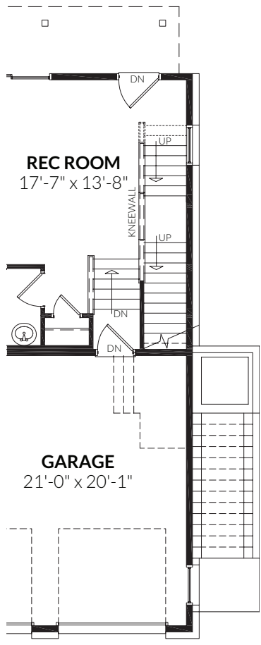
GROUND LEVEL WITH DROPPED BASEMENT (END UNIT)
