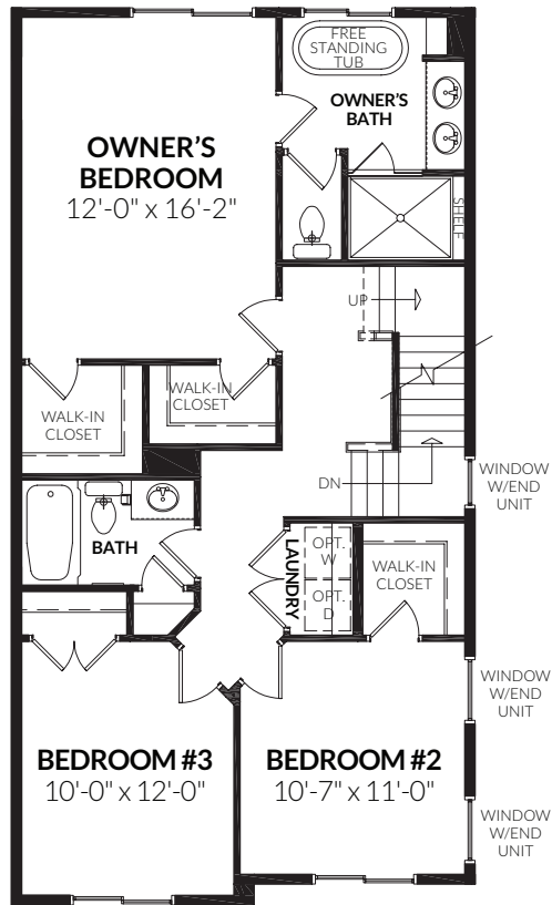
SECOND FLOOR (INTERIOR UNIT)
