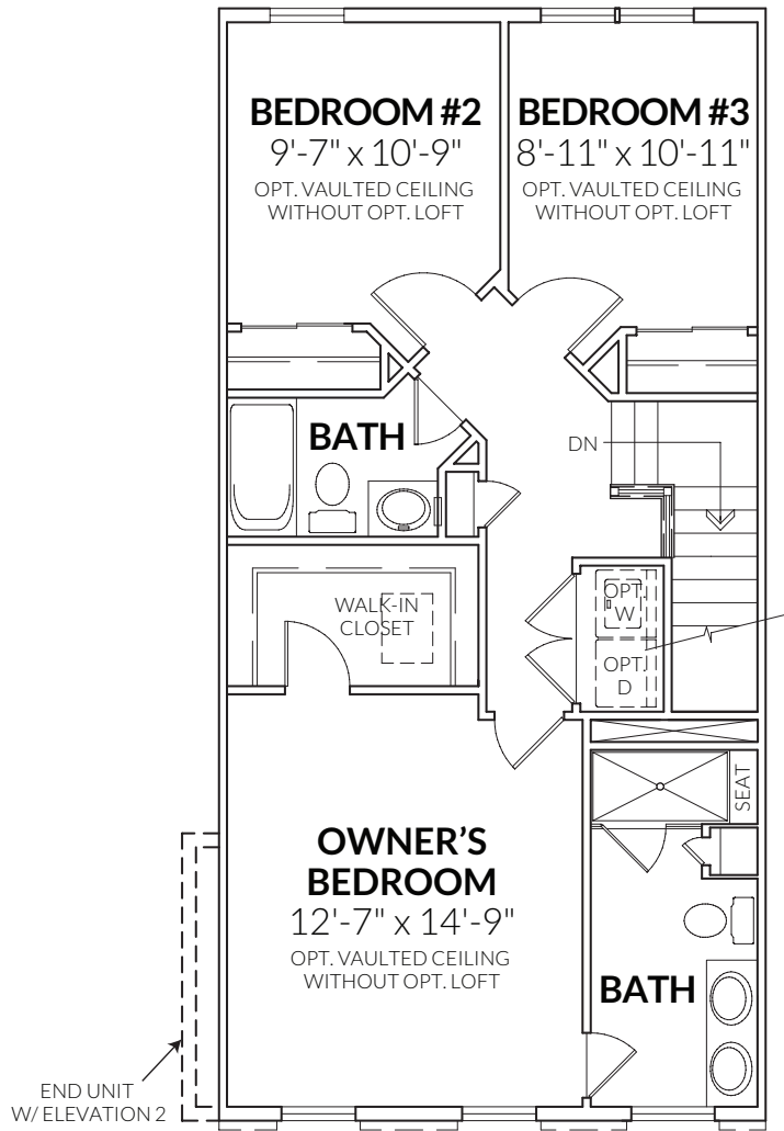
STANDARD SECOND FLOOR
