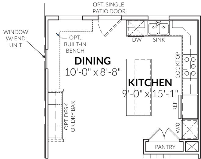
ALTERNATE FIRST FLOOR
