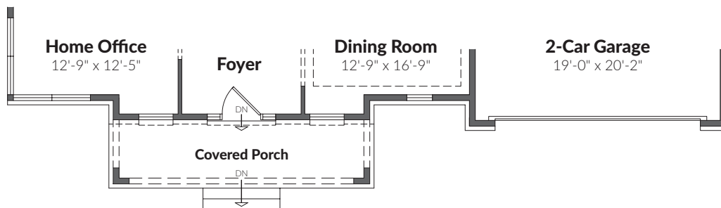
FIRST FLOOR SHOWN WITH ELEVATION 4
