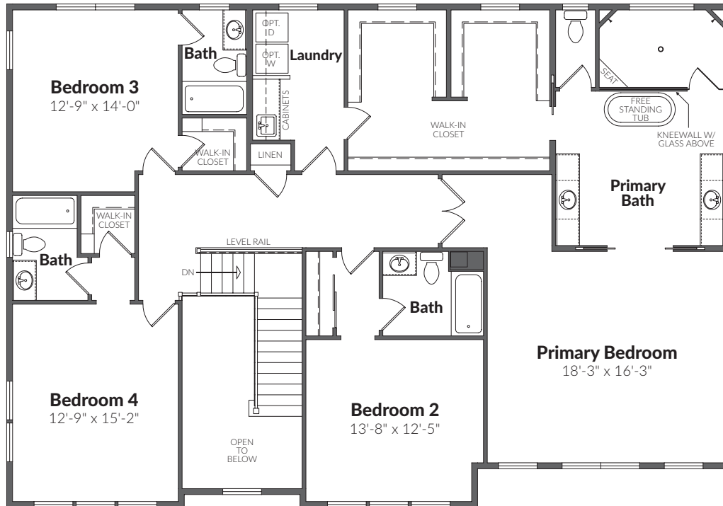
SECOND FLOOR SHOWN WITH ELEVATION 2
