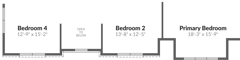
SECOND FLOOR SHOWN WITH ELEVATION 3
