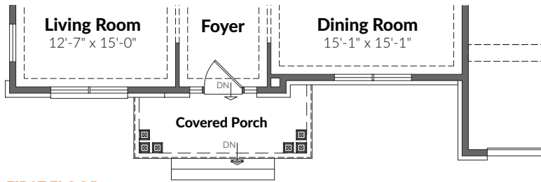
FIRST FLOOR SHOWN WITH ELEVATION 2
