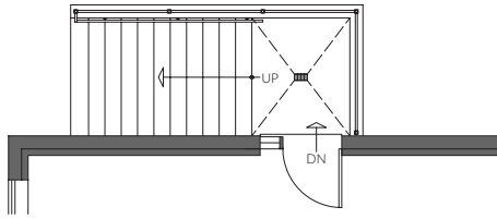
BASEMENT WITH OPT. WELLED EXIT "C"
