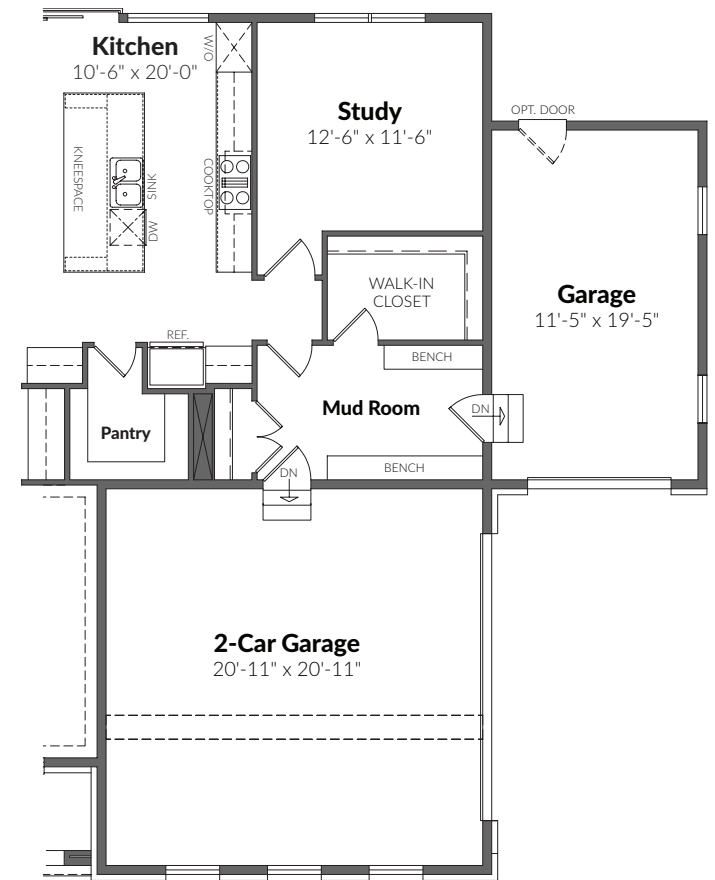
FIRST FLOOR WITH OPT. 3-CAR SIDE-LOAD GARAGE
