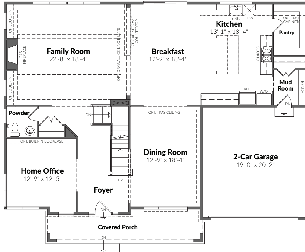
FIRST FLOOR SHOWN WITH ELEVATION 1
