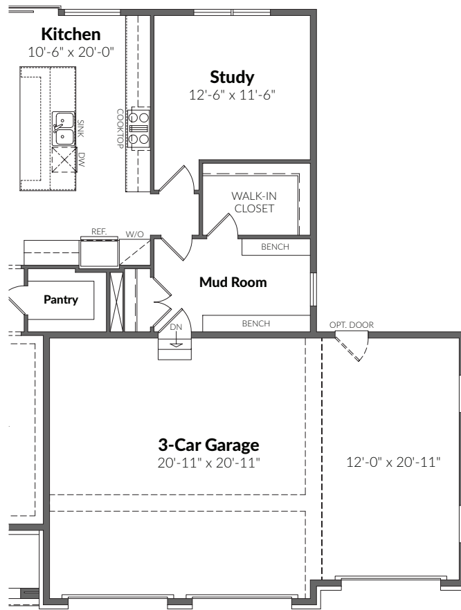
FIRST FLOOR OPT. 3-CAR FRONT-LOAD GARAGE
