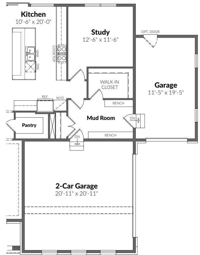
FIRST FLOOR WITH OPT. 3-CAR SIDE-LOAD GARAGE
