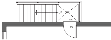
BASEMENT WITH OPT. WELLED EXIT "A"
