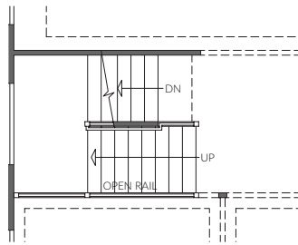
FIRST FLOOR WITH OPT. OPEN RAIL
